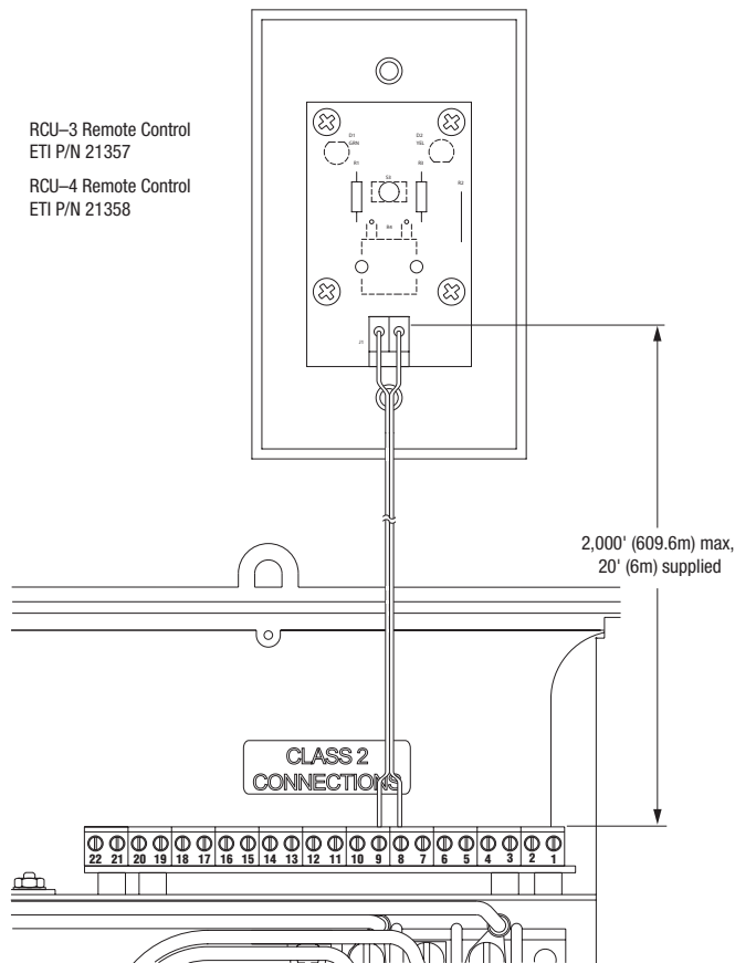
Fig 1: RCU-3 and RCU-4 remote connections to C-series panels.
